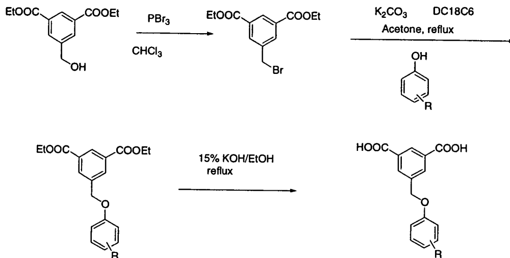
Scheme I-B
